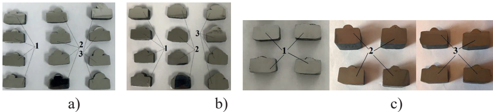
Figure 3. Samples after grinding: a - STODY M7-G; b - STODY 102-G; c - TUBRODUR 58 O / G M; 1 - single-layer surfacing; 2- two-layer surfacing; 3 - three-layer surfacing
